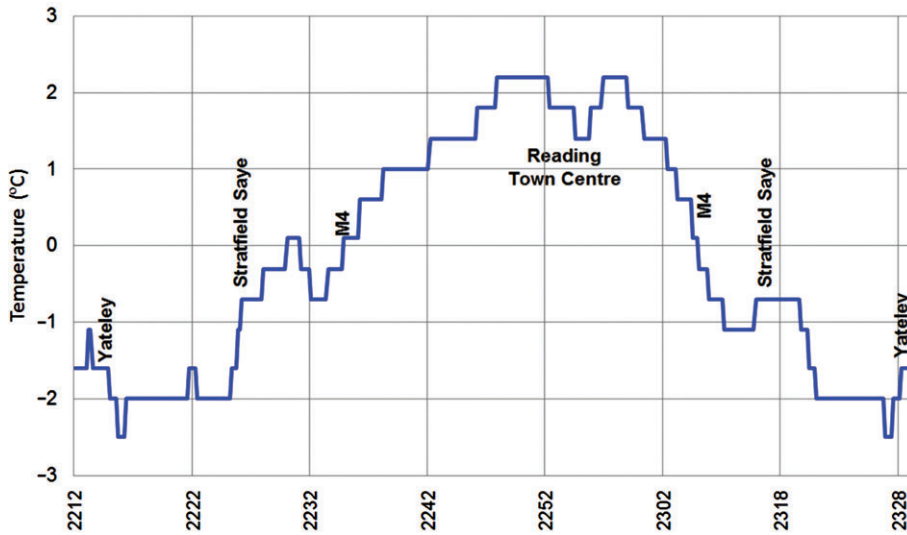
Figure 10. The heat island effect of Reading, 18 February 2013. A temperature cross-section going from the surrounding countryside into the town centre and back out again, with times in UTC.
