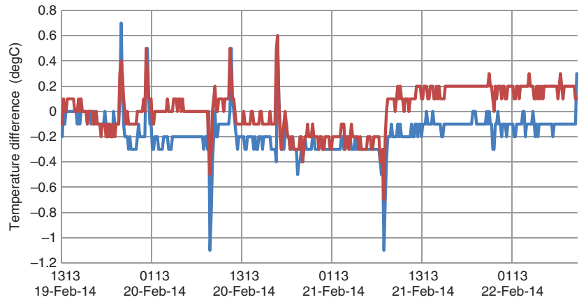
Figure 3. Temperature differences between one of the loggers (arbitrarily chosen as a reference) and the other two, during the same period as in Figure 2.
