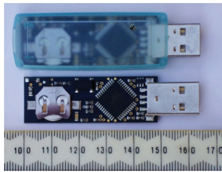
Figure 1. The temperature logger as supplied (top) showing the ventilation hole in the top right corner, and with casing removed (bottom): scale in mm.
