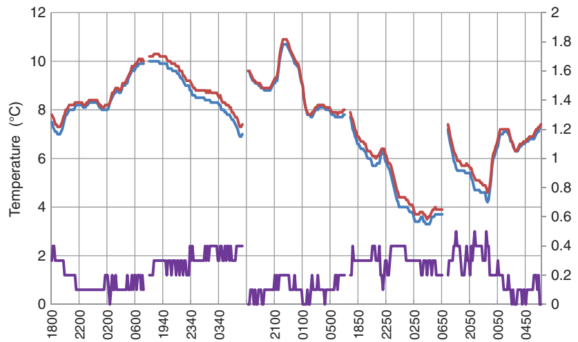
Figure 4. Temperature from the logger (blue) and Davis VP2 weather station (red) over the five nights 22–27 February 2014, and the difference (degC) between them (purple, right-hand scale): times in UTC.
