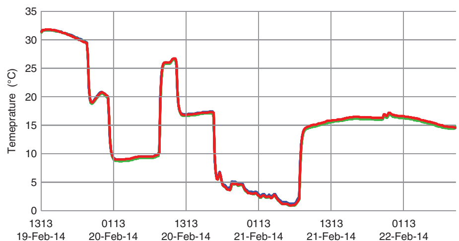
Figure 2. Temperature traces from three loggers over the period 19–22 February 2014, with times in UTC.
