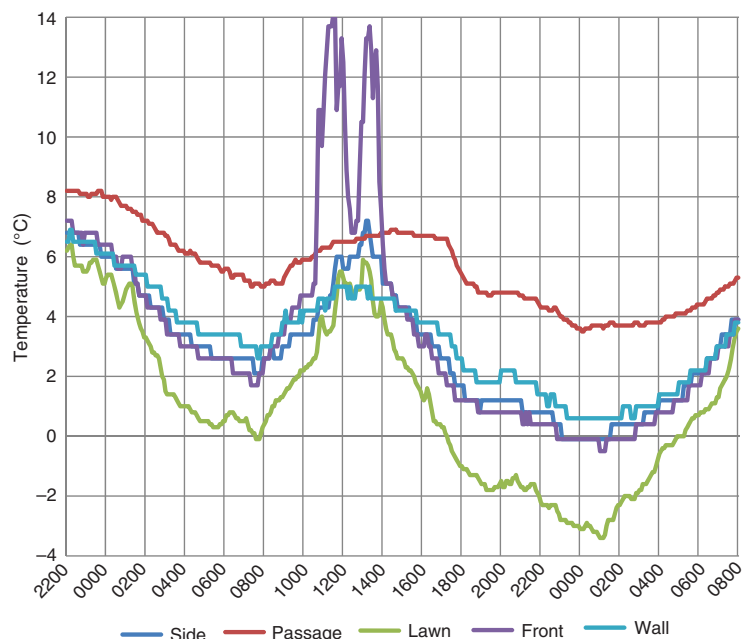
Figure 5. Temperature over the period 2200 UTC on 18 November to 0800 UTC on 20 November 2013 (times in UTC), at five locations around a house and garden. The spikes on the 'Front' (purple) trace are where direct solar radiation has heated up the container, and hence the air around the sensor, well above ambient air temperature.
