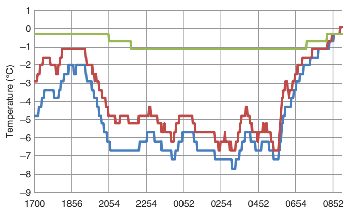
Figure 6. Temperature versus time of day (UTC) on grass under snow (green), on the surface of the snow (blue) and on a cleared area of grass (red), during the night of 20/21 January 2013.
