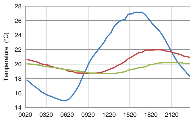
Figure 8. The air temperature at a height of 1.2m (blue) and soil temperatures at depths of 10cm (red) and 20cm (green) below a grass surface, averaged over the 8 day period shown in Figure 7: times in UTC.
