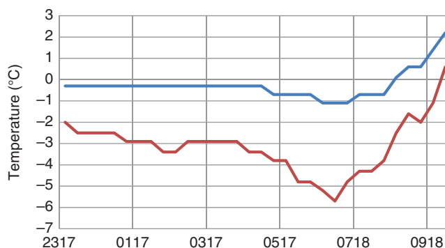
Figure 9. Temperatures during the night of 6/7 February 2013 (times in UTC) at the surface of a lawn open to the sky (red) and nearby but covered with a garden fleece (blue).
