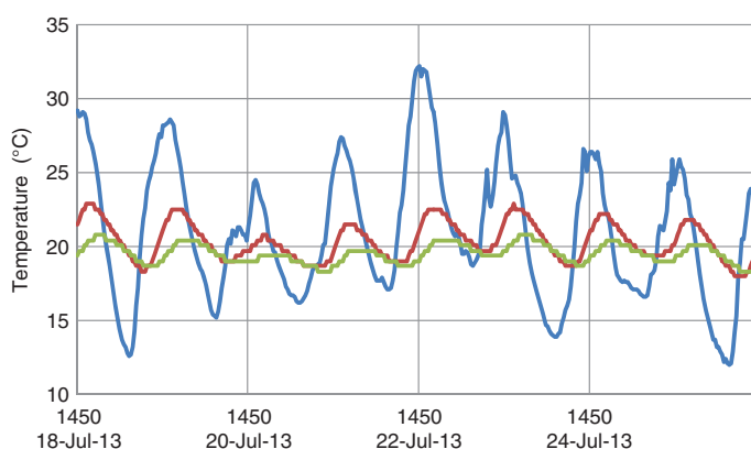
Figure 7. The air temperature at a height of 1.2m (blue) and soil temperatures at depths of 10cm (red) and 20cm (green) below a grass surface: times in UTC.
