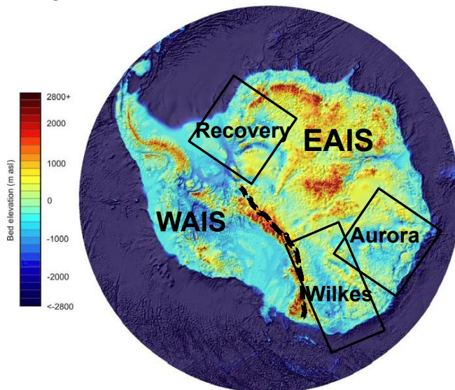
Figure 1. Antarctica with its two major ice sheets, the West and East Antarctic Ice Sheets (WAIS, EAIS). Three large sub-glacial basins in the EAIS are labelled.
